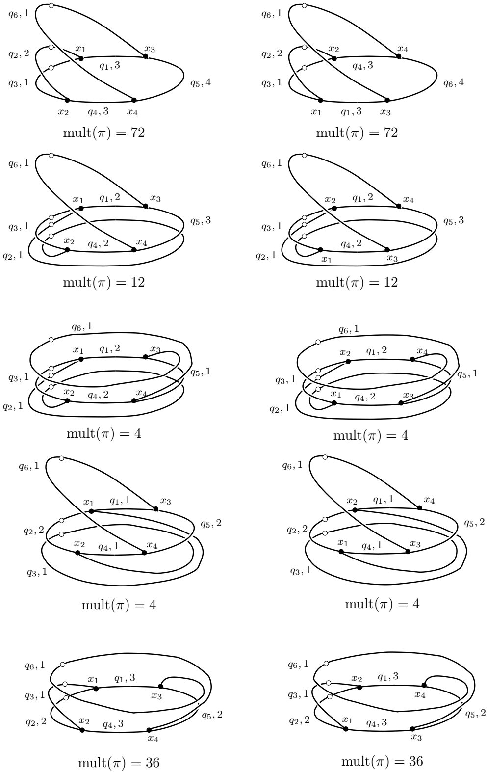
FIGURE 4. All labeled tropical covers contributing to N_{(0,2,1,0,0,1),\Gamma}^{\text{trop}} = 256 .
